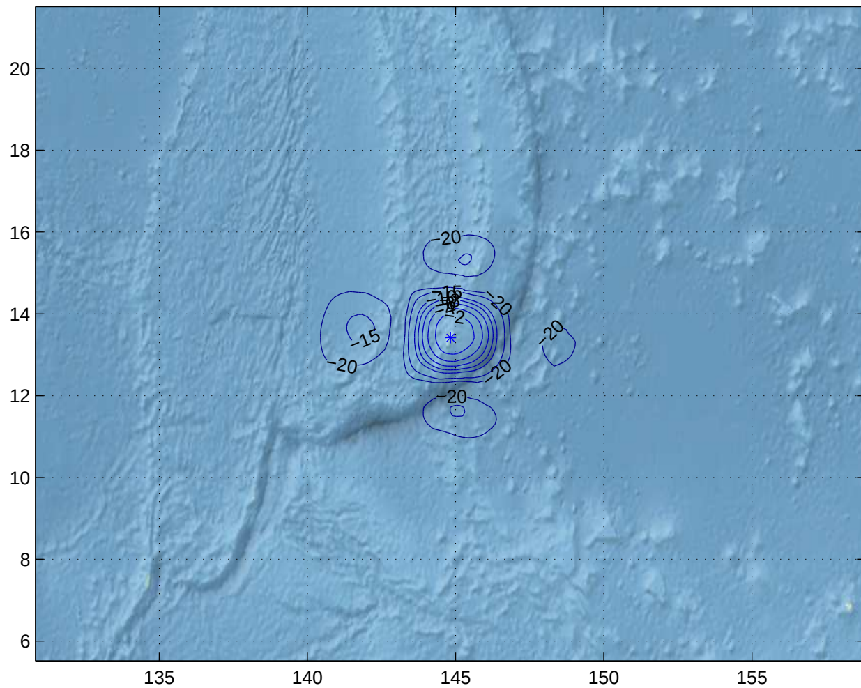
Gain Contours at 450km for GUM. Beam ID=XTC, Polarization=rhcp
