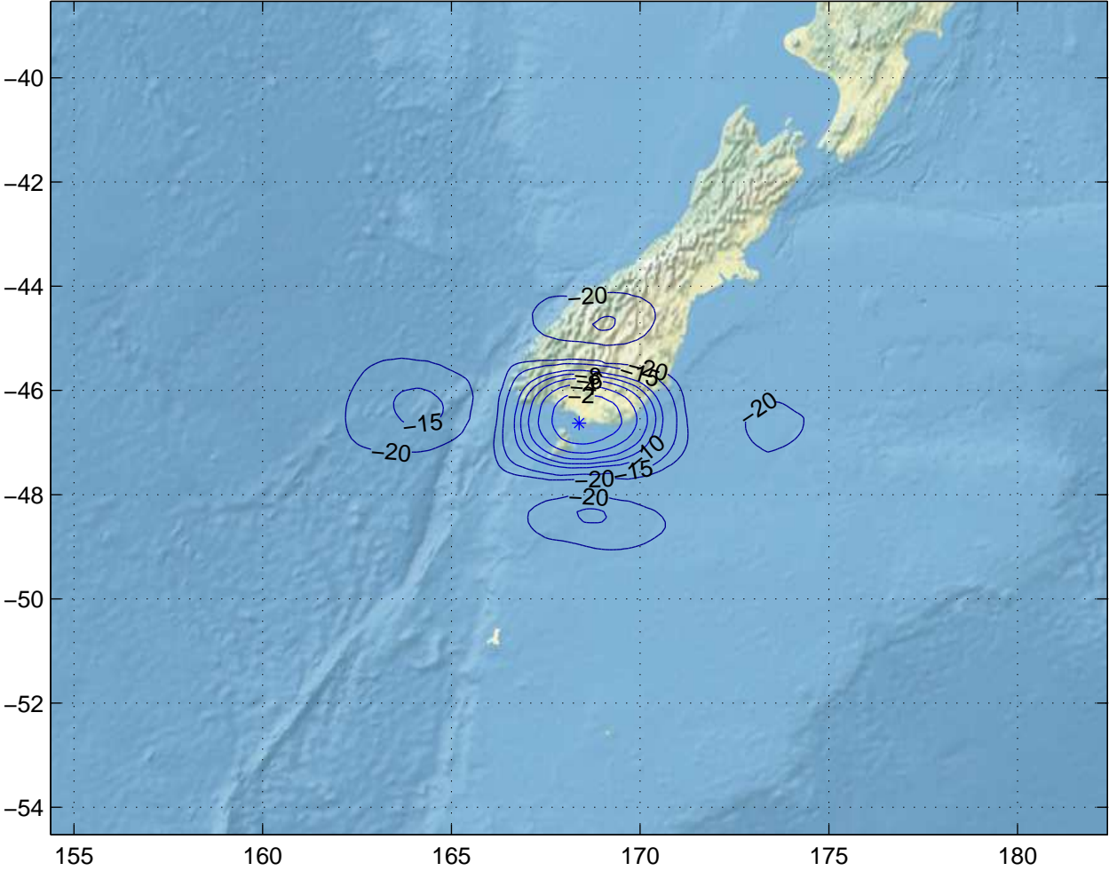
Gain Contours at 450km for IVC. Beam ID=XTC, Polarization=rhcp
