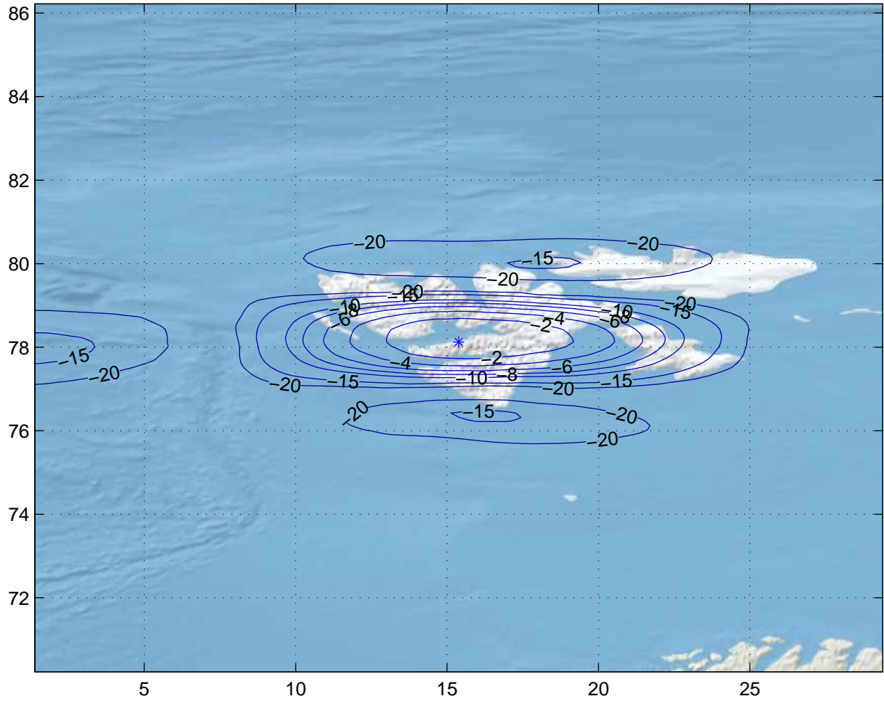
Gain Contours at 450km for LYR. Beam ID=XTC, Polarization=rhcp
