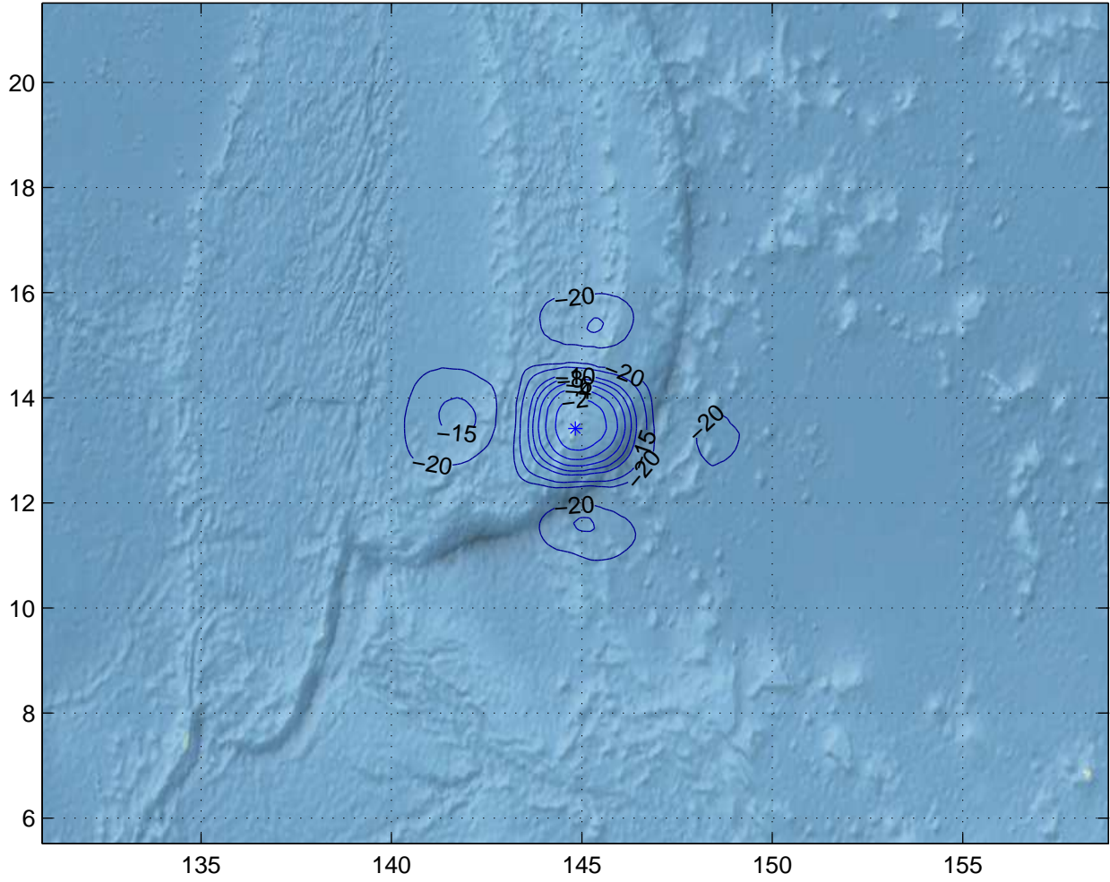
Gain Contours at 460km for GUM. Beam ID=XTC, Polarization=rhcp
