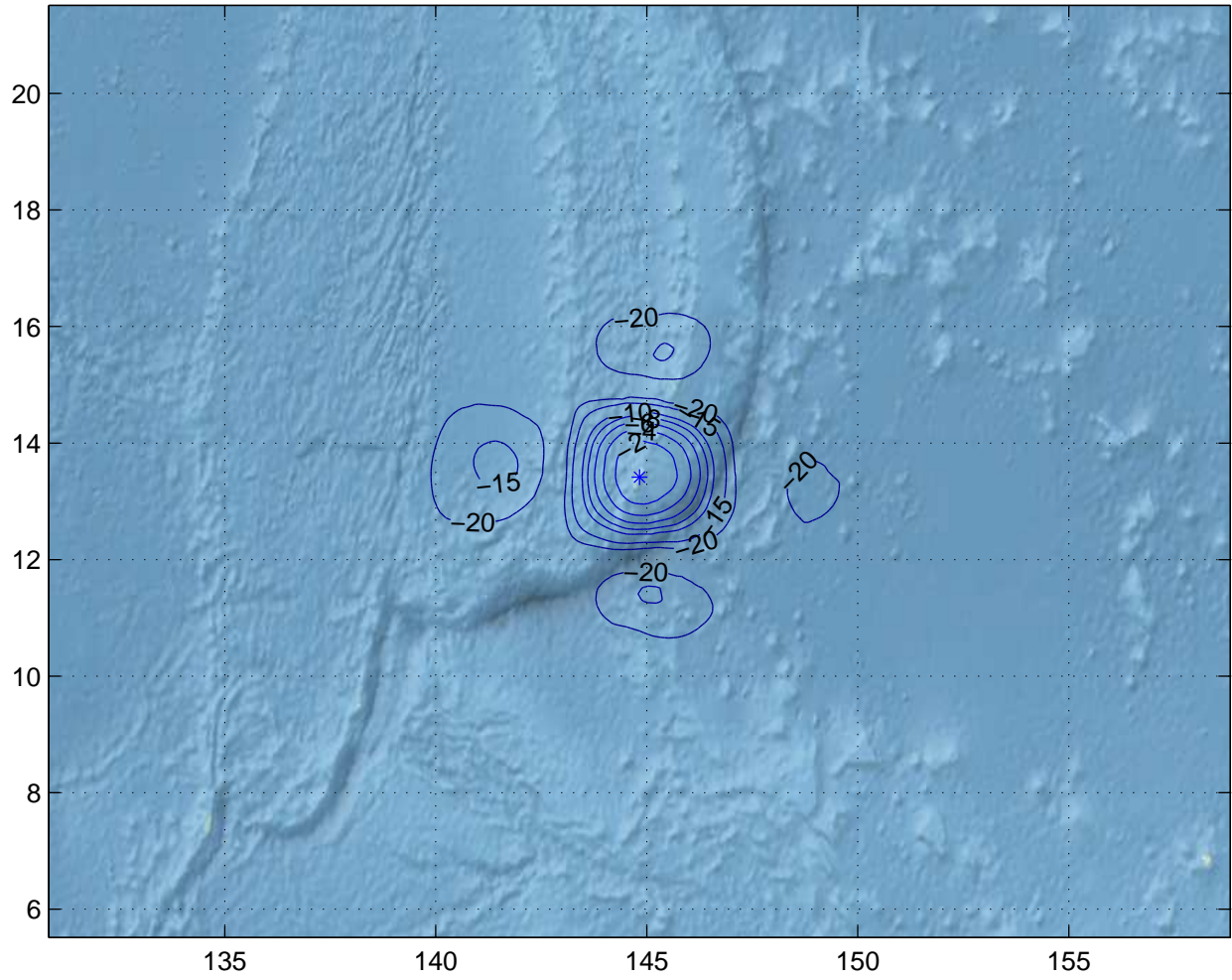
Gain Contours at 505km for GUM. Beam ID=XTC, Polarization=rhcp
