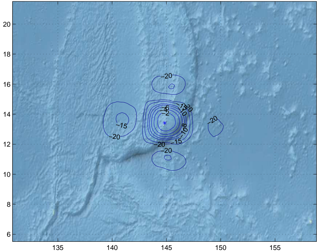
Gain Contours at 575km for GUM. Beam ID=XTC, Polarization=rhcp
