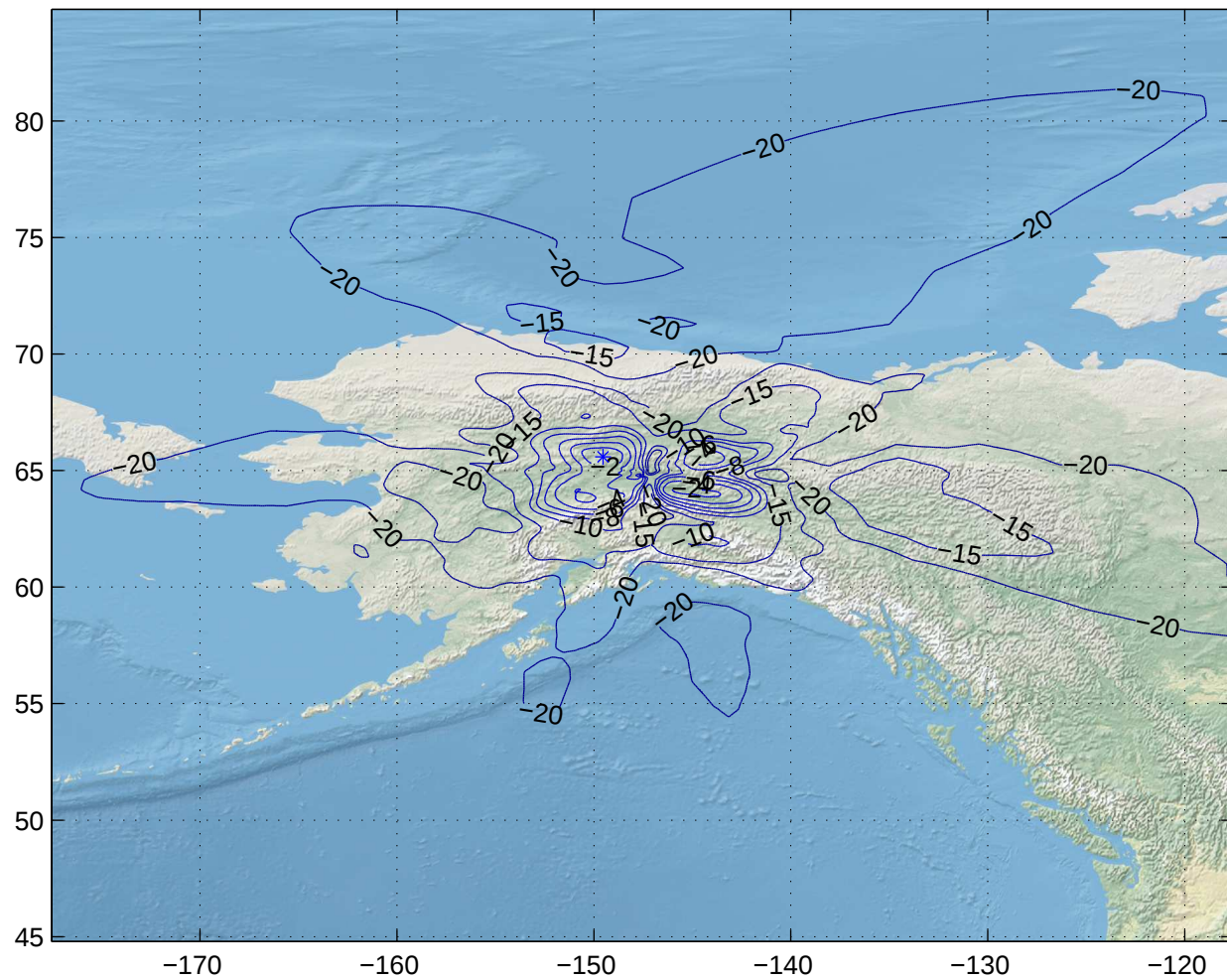
Gain Contours at 450km for FAI. Beam ID=XTX, Polarization=lhcp
