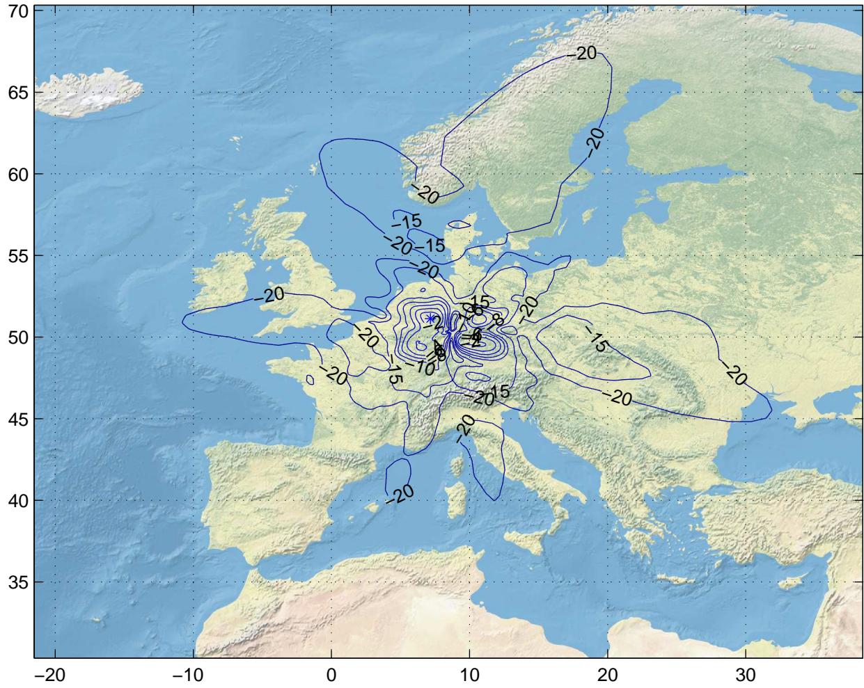
Gain Contours at 450km for FRA. Beam ID=XTX, Polarization=lhcp
