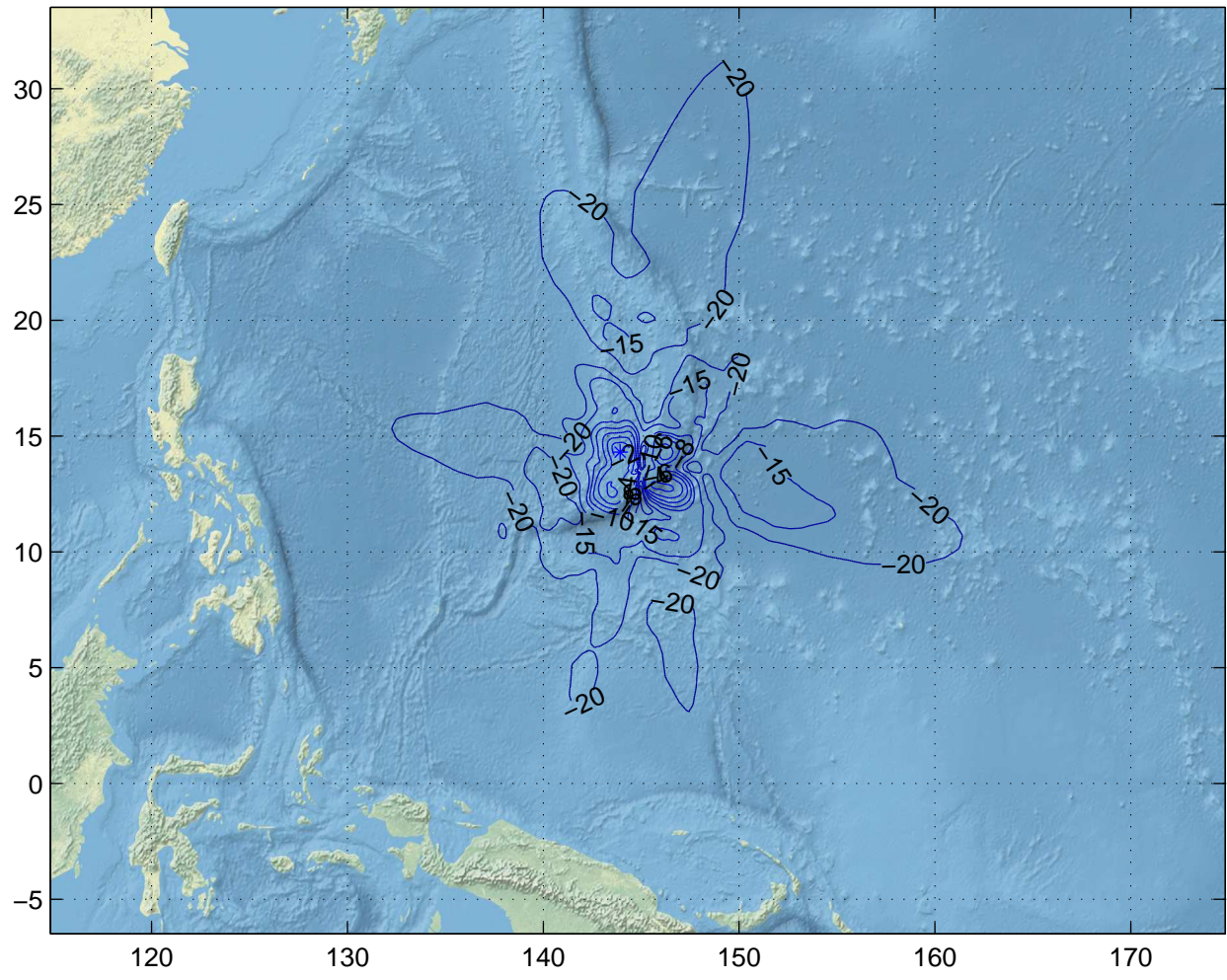
Gain Contours at 450km for GUM. Beam ID=XTX, Polarization=lhcp
