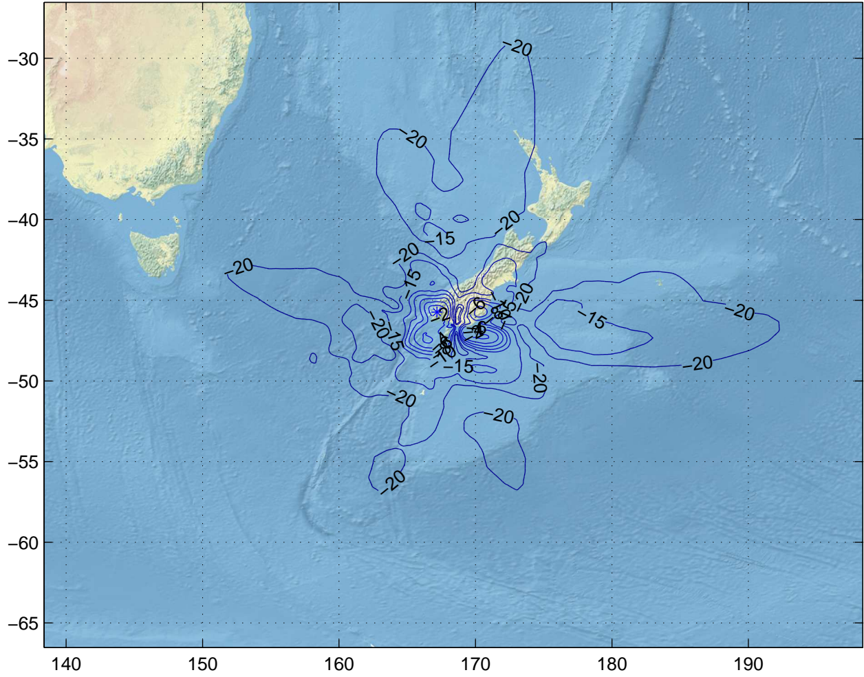
Gain Contours at 450km for IVC. Beam ID=XTX, Polarization=lhcp
