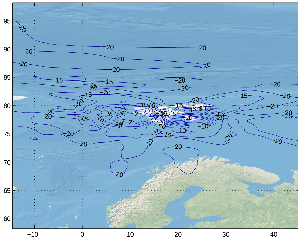
Gain Contours at 450km for LYR. Beam ID=XTX, Polarization=lhcp
