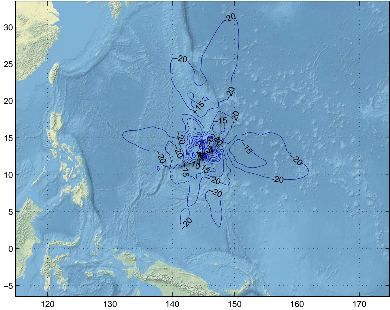
Gain Contours at 460km for GUM. Beam ID=XTX, Polarization=lhcp
