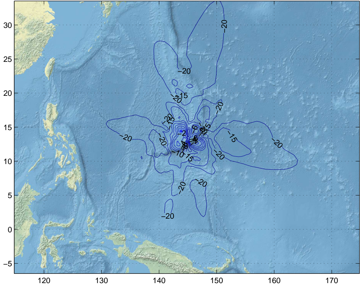
Gain Contours at 505km for GUM. Beam ID=XTX, Polarization=lhcp
