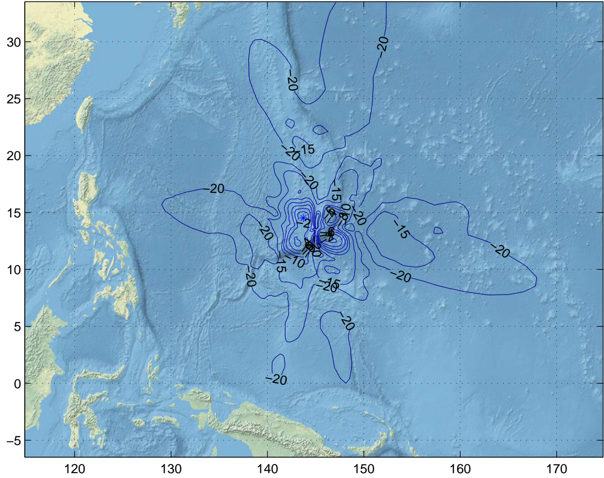
Gain Contours at 575km for GUM. Beam ID=XTX, Polarization=lhcp
