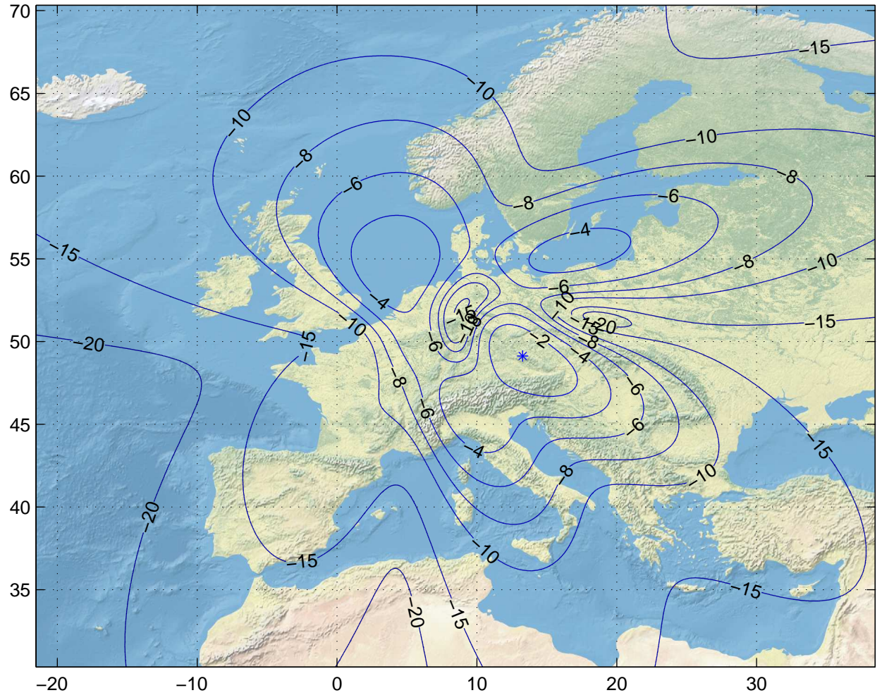
Gain Contours at 575km for FRA. Beam ID=URX, Polarization=rhcp
