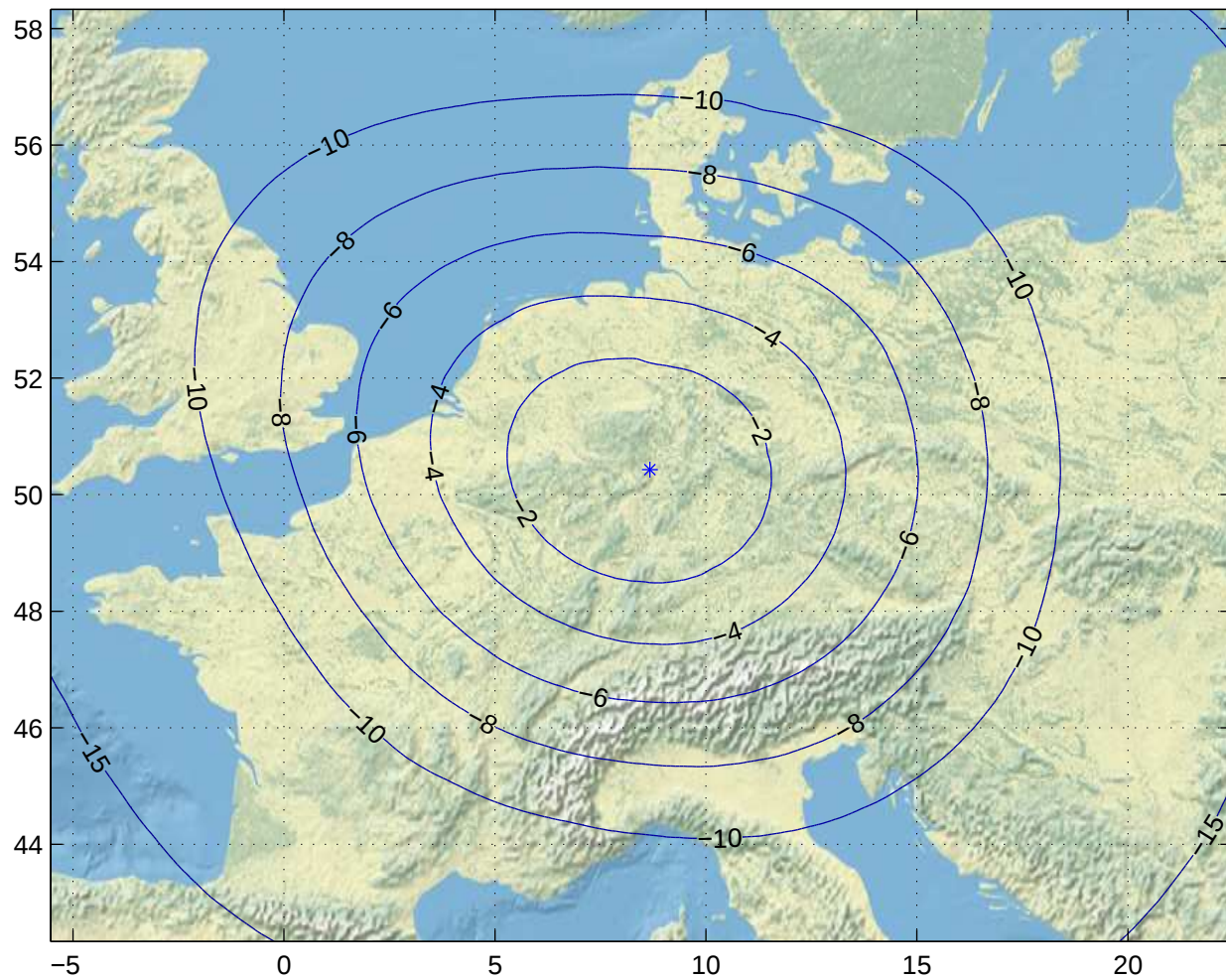
Gain Contours at 450km for FRA. Beam ID=SRC, Polarization=rhcp
