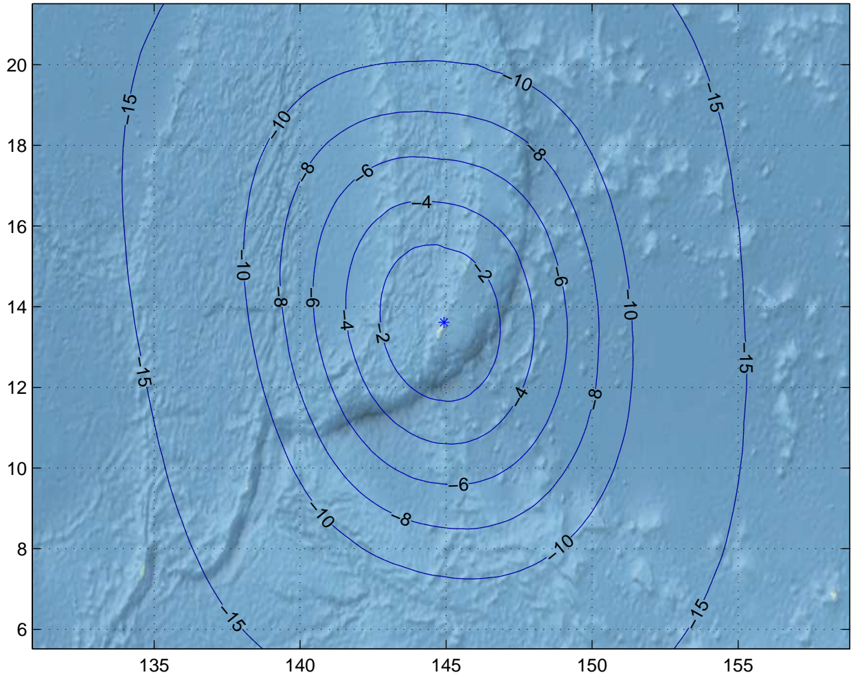
Gain Contours at 450km for GUM. Beam ID=SRC, Polarization=rhpc
