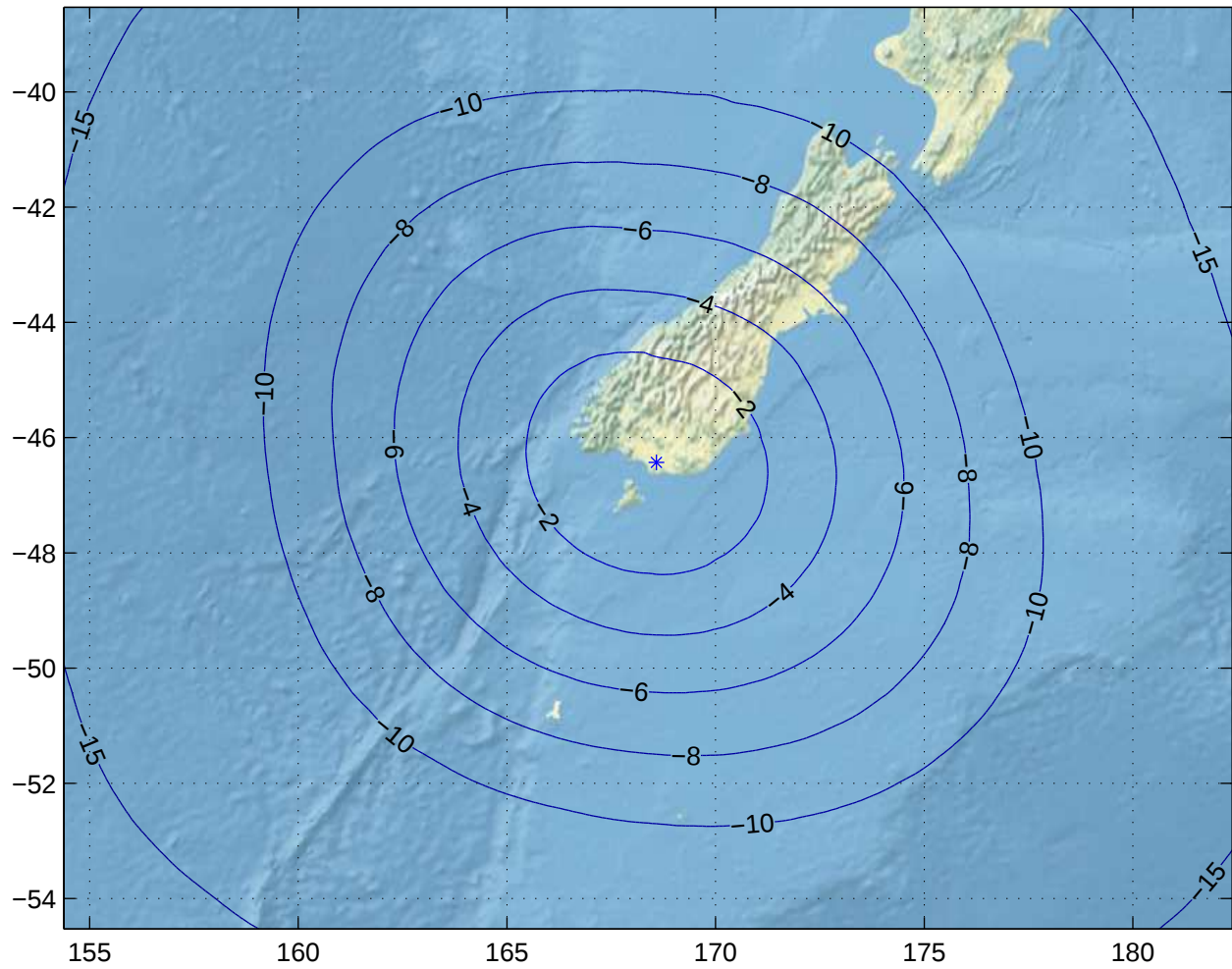
Gain Contours at 450km for IVC. Beam ID=SRC, Polarization=rhcp
