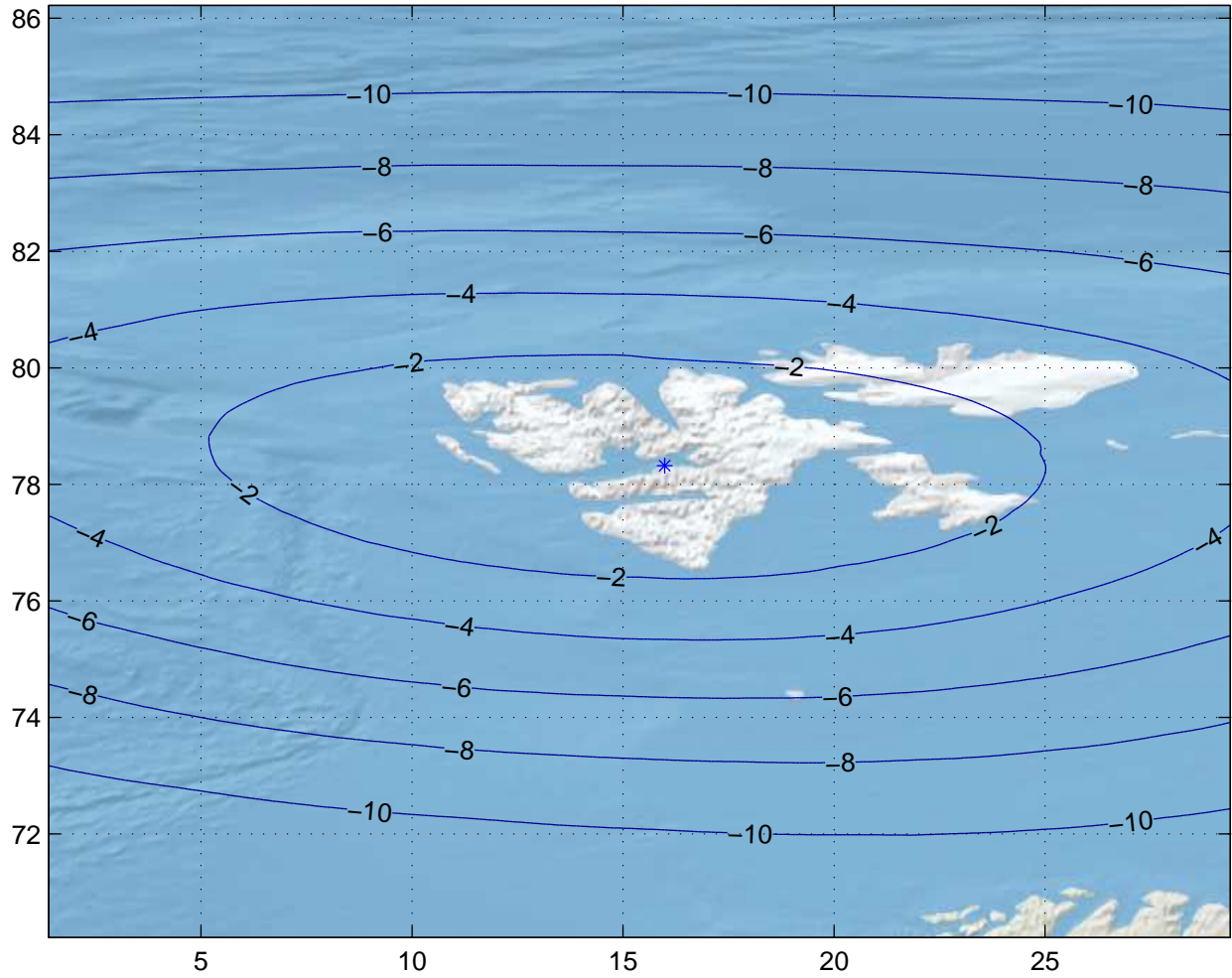
Gain Contours at 450km for LYR. Beam ID=SRC, Polarization=rhcp
