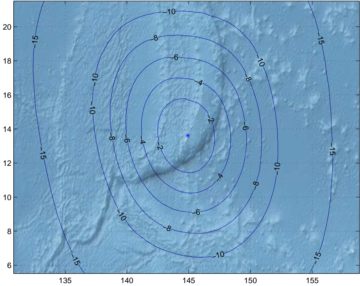
Gain Contours at 505km for GUM. Beam ID=SRC, Polarization=rhcp
