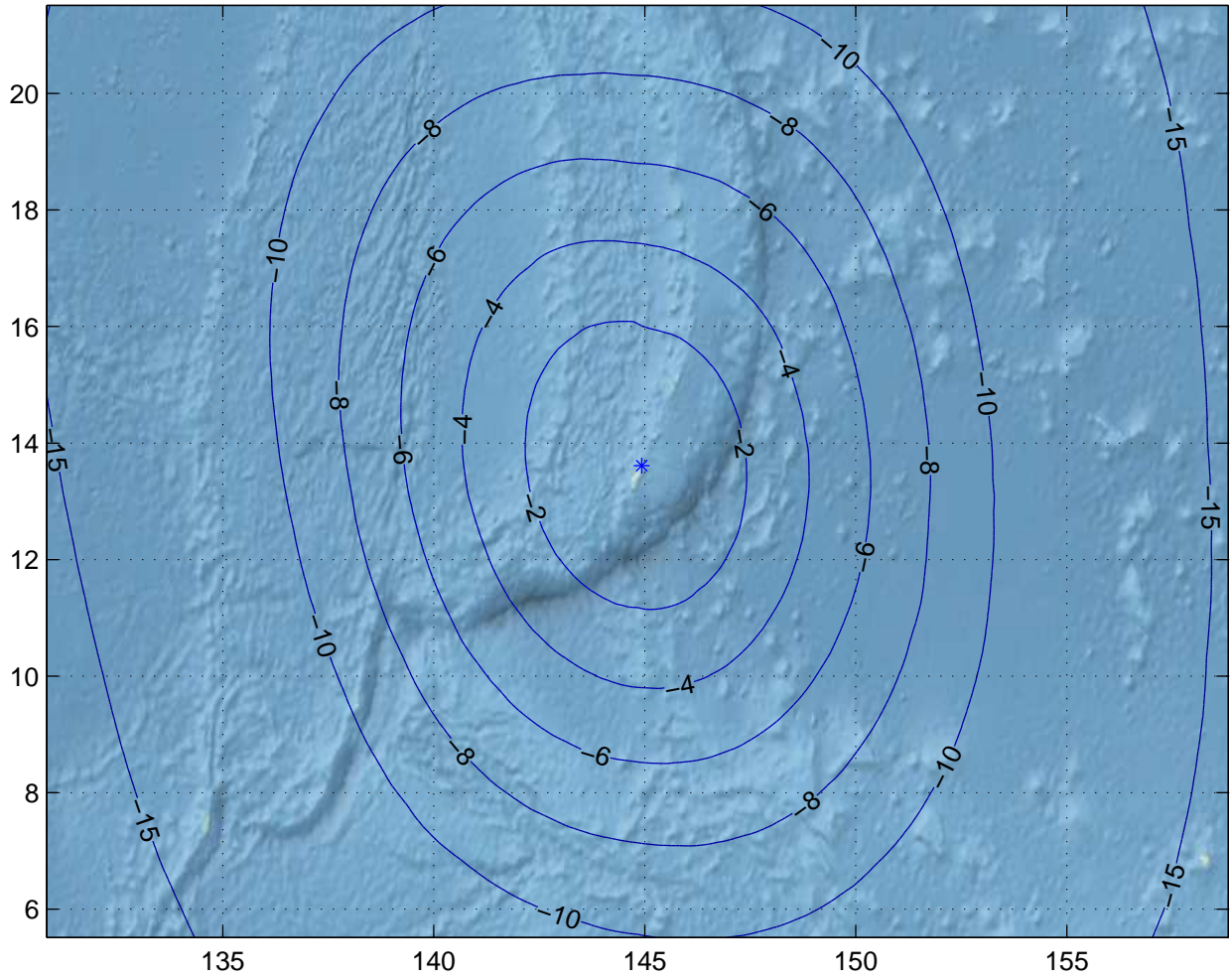
Gain Contours at 575km for GUM. Beam ID=SRC, Polarization=rhcp
