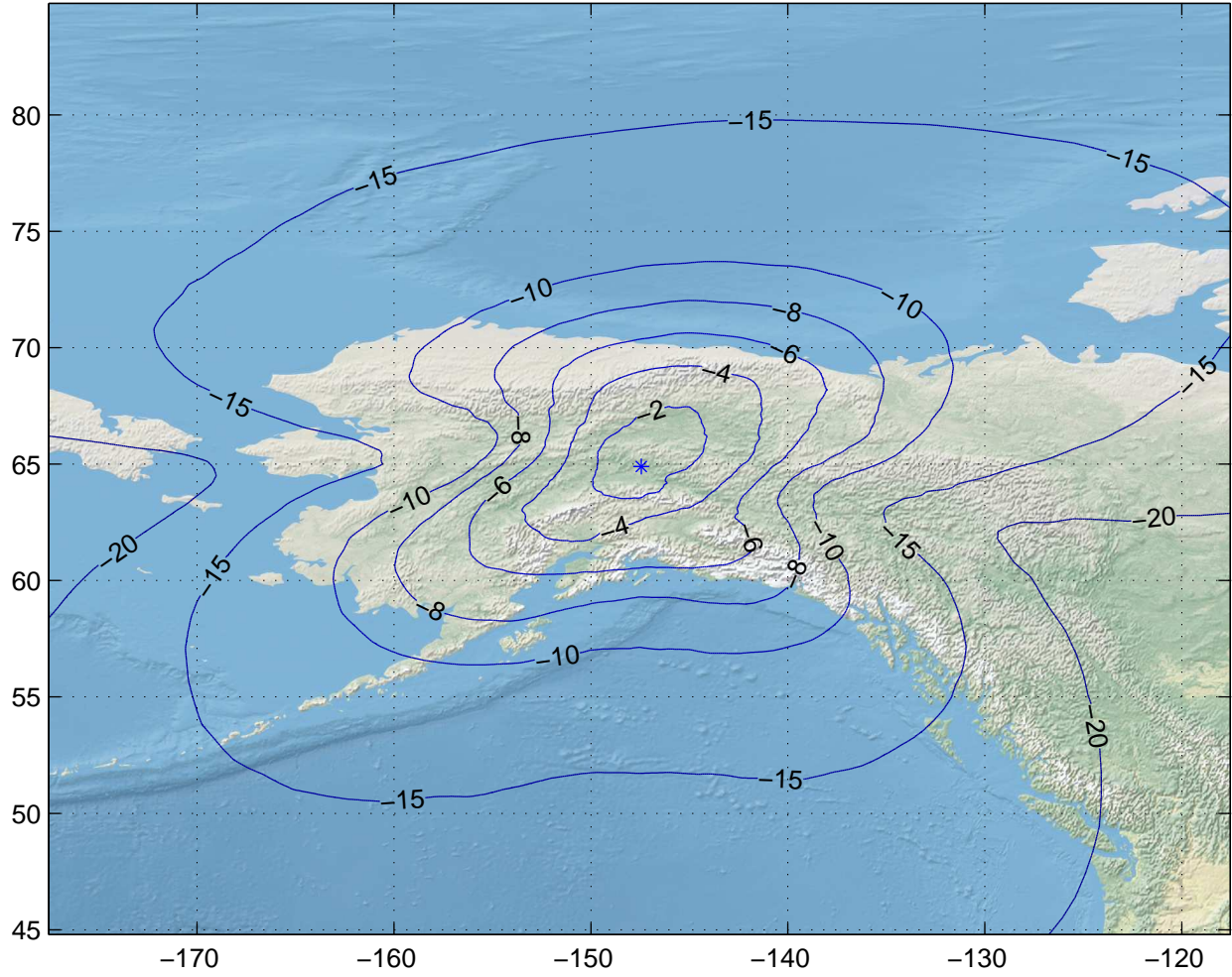
Gain Contours at 450km for FAI. Beam ID=SRX, Polarization=lhcp
