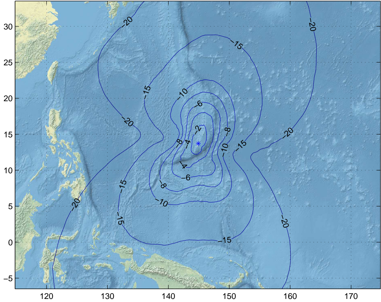
Gain Contours at 450km for GUM. Beam ID=SRX, Polarization=lhcp
