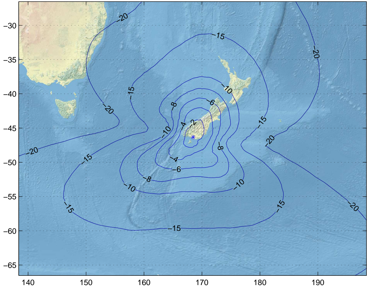
Gain Contours at 450km for IVC. Beam ID=SRX, Polarization=lhcp
