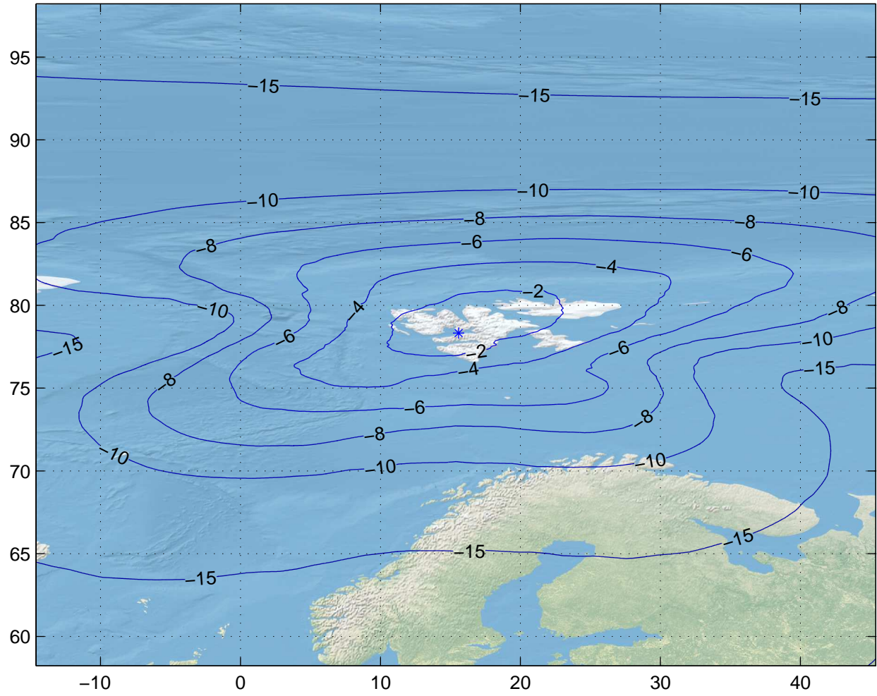
Gain Contours at 450km for LYR. Beam ID=SRX, Polarization=lhcp
