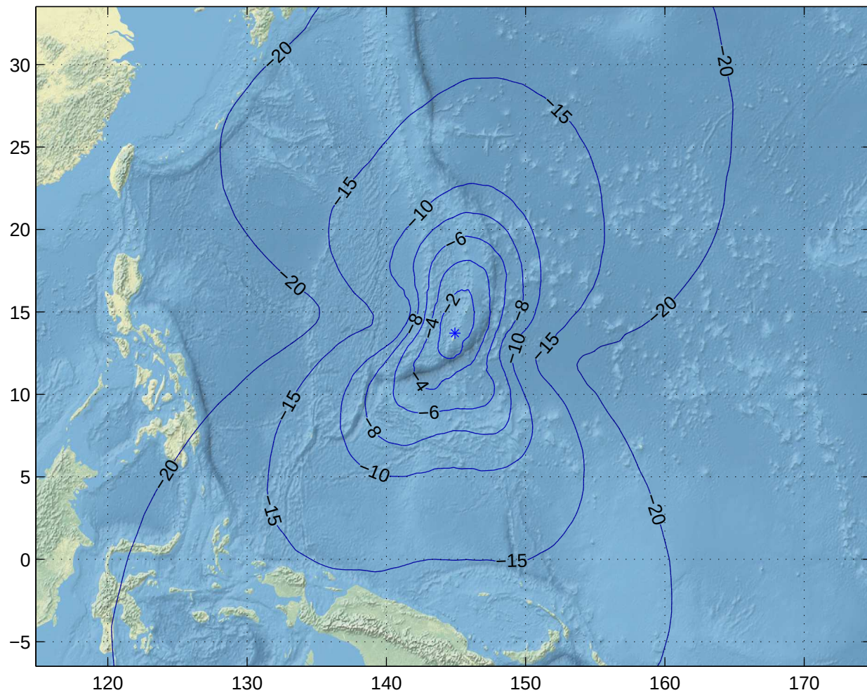
Gain Contours at 460km for GUM. Beam ID=SRX, Polarization=lhcp
