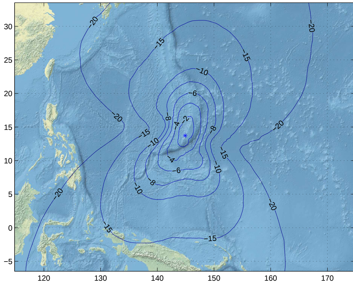
Gain Contours at 505km for GUM. Beam ID=SRX, Polarization=lhcp
