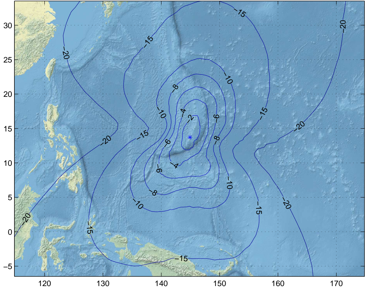
Gain Contours at 575km for GUM. Beam ID=SRX, Polarization=lhpc
