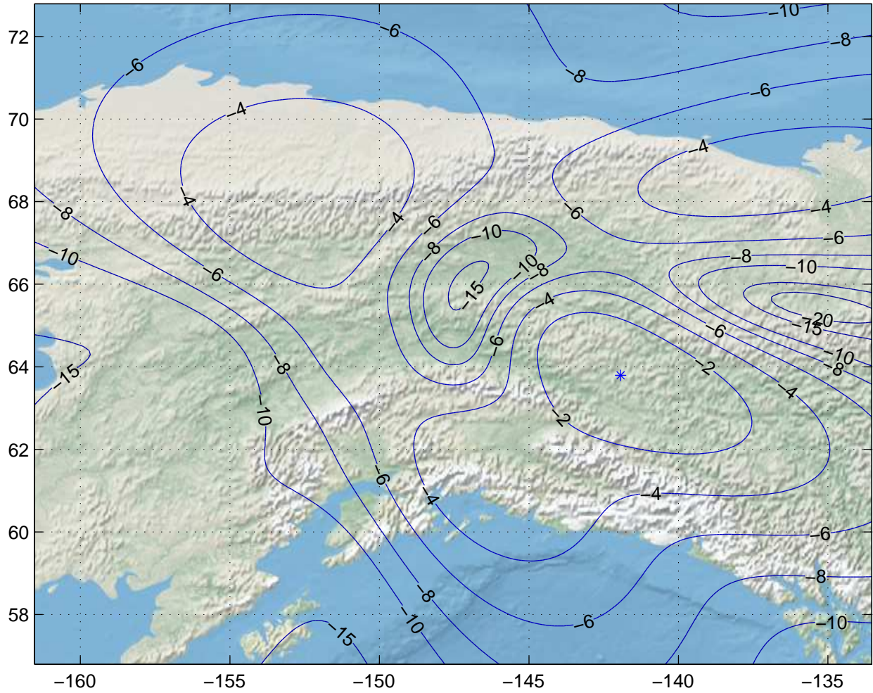
Gain Contours at 450km for FAI. Beam ID=URC, Polarization=h
