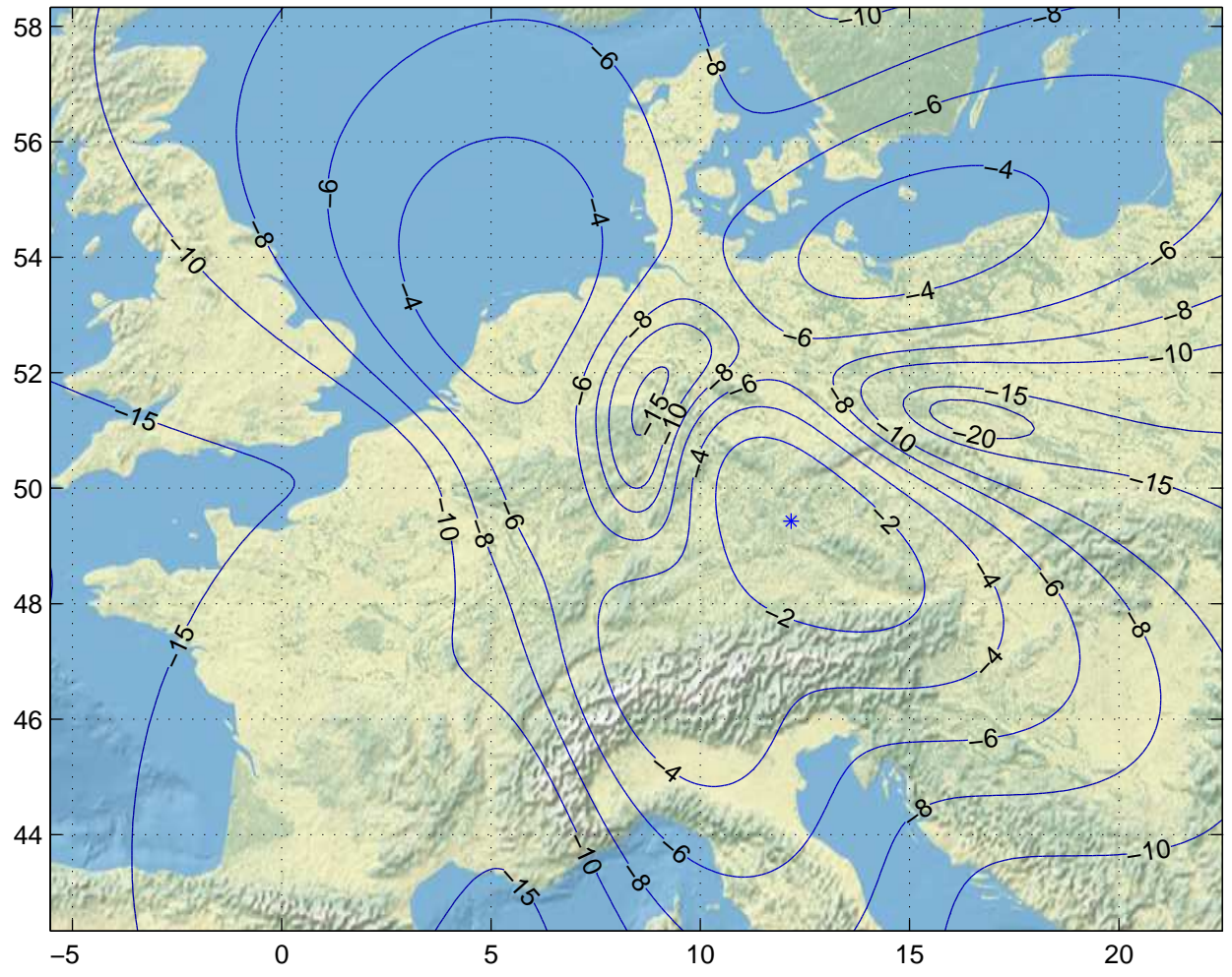
Gain Contours at 450km for FRA. Beam ID=URC, Polarization=h
