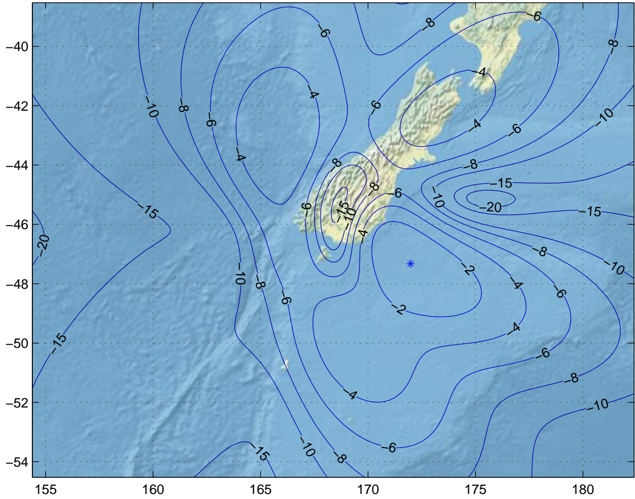
Gain Contours at 450km for IVC. Beam ID=URC, Polarization=h
