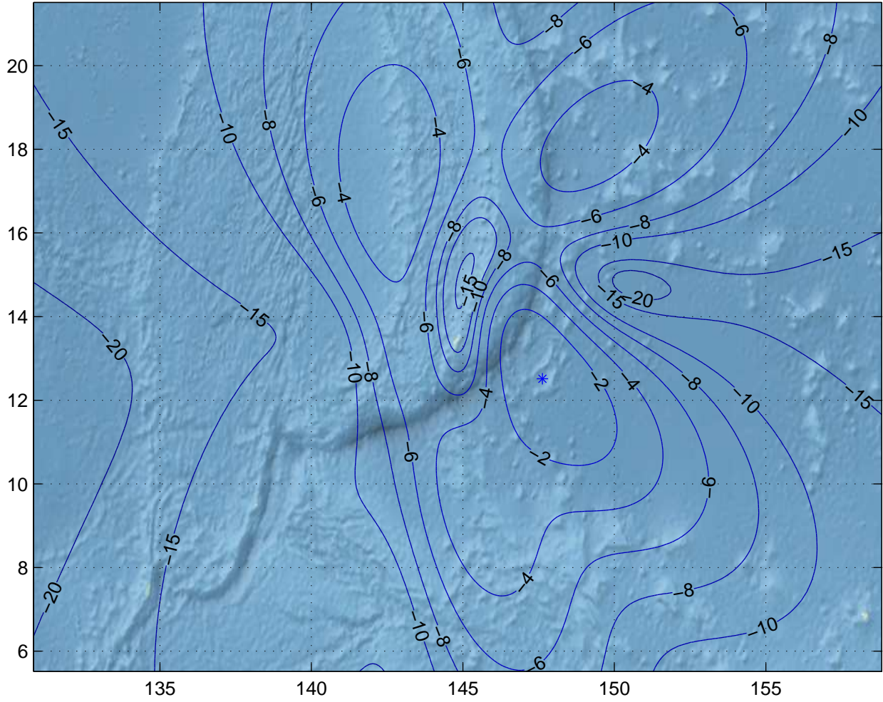
Gain Contours at 505km for GUM. Beam ID=URC, Polarization=h
