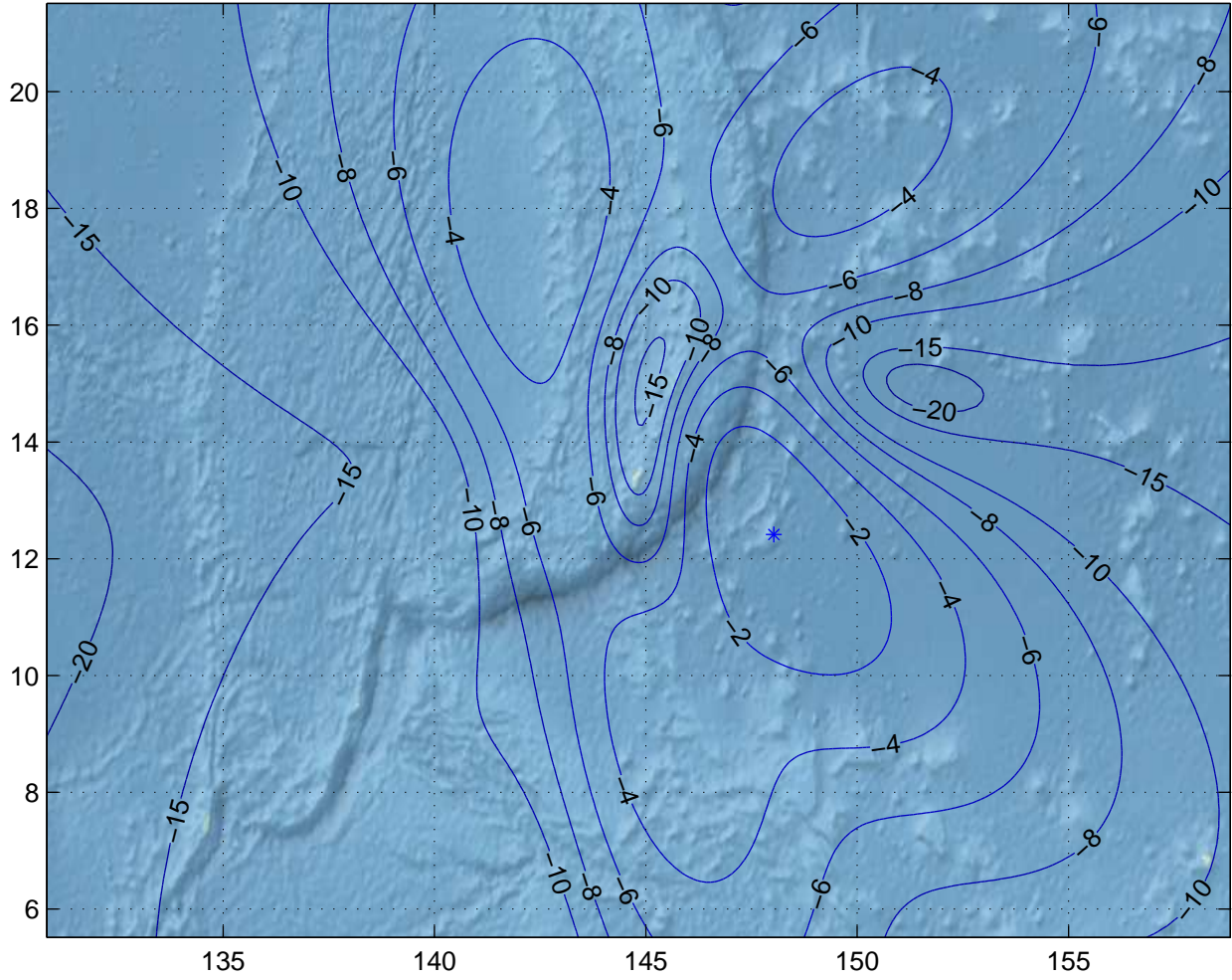
Gain Contours at 575km for GUM. Beam ID=URC, Polarization=h
