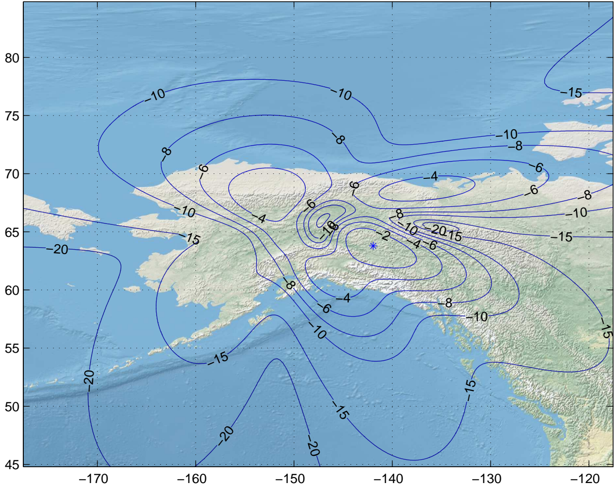
Gain Contours at 450km for FAI. Beam ID=URX, Polarization=rhcp
