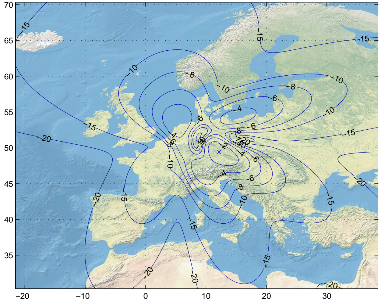
Gain Contours at 450km for FRA. Beam ID=URX, Polarization=rhcp
