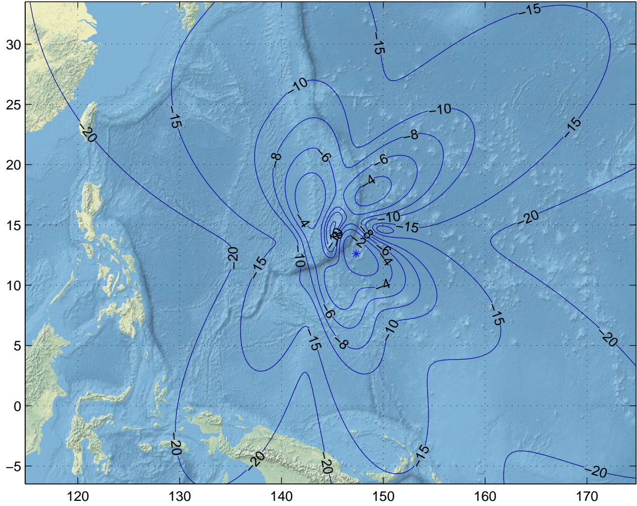
Gain Contours at 450km for GUM. Beam ID=URX, Polarization=rhcp
