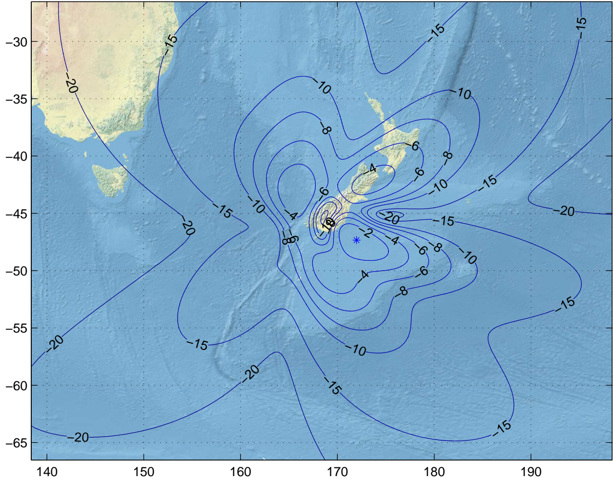
Gain Contours at 450km for IVC. Beam ID=URX, Polarization=rhcp
