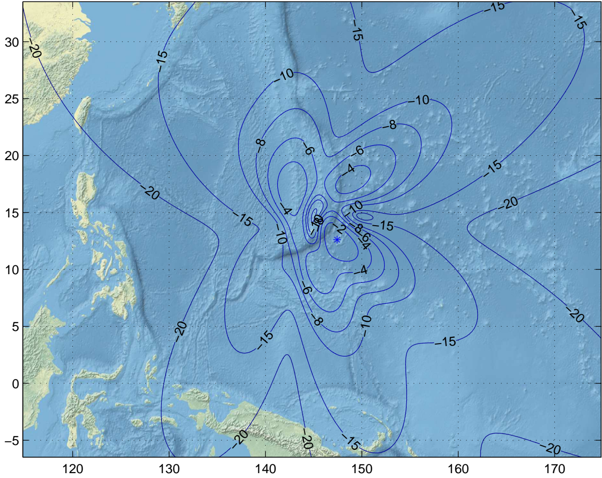
Gain Contours at 460km for GUM. Beam ID=URX, Polarization=rhcp
