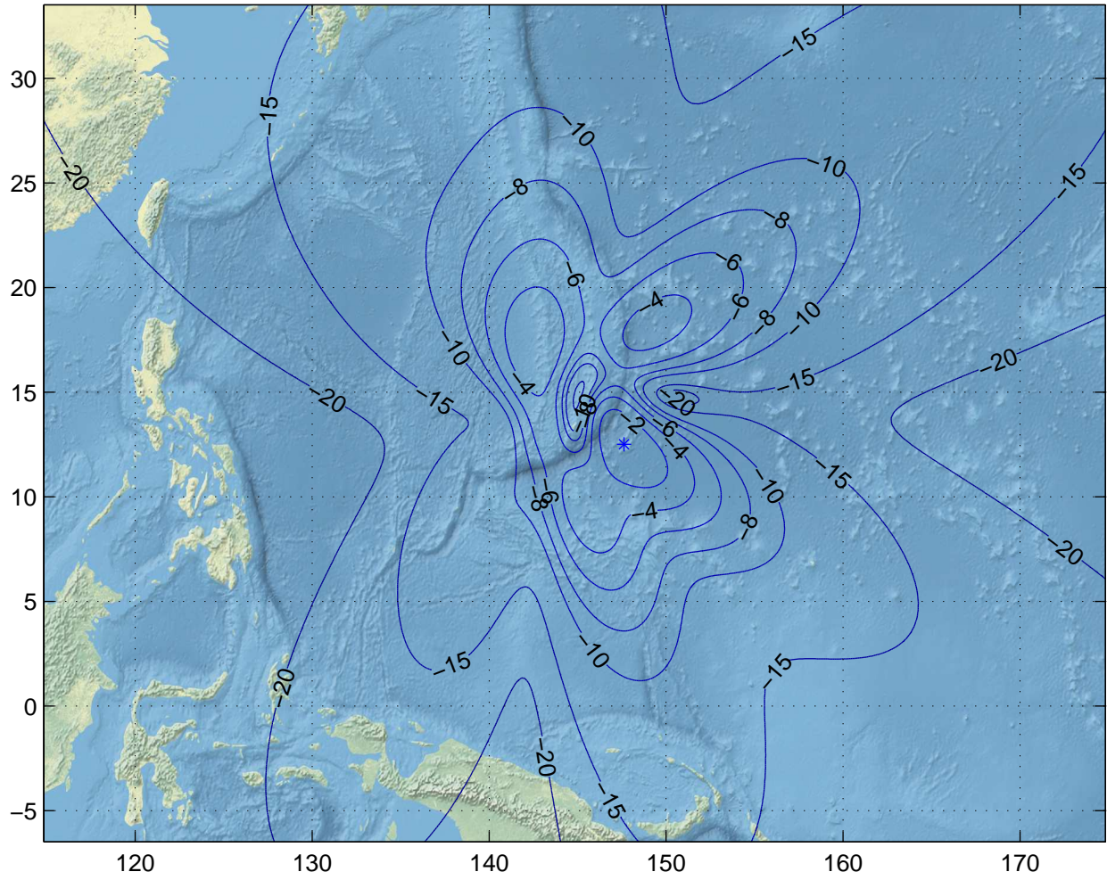
Gain Contours at 505km for GUM. Beam ID=URX, Polarization=rhcp
