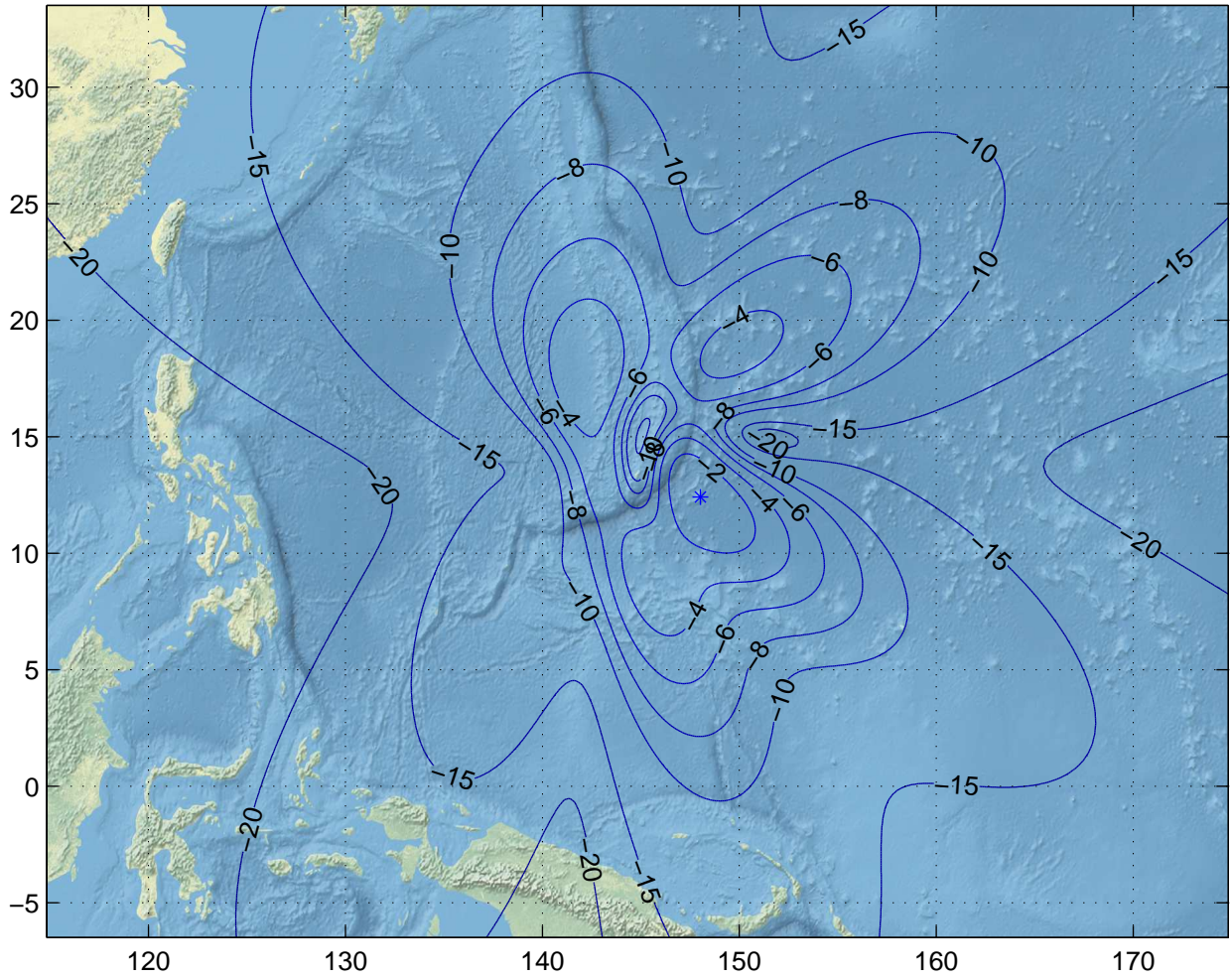
Gain Contours at 575km for GUM. Beam ID=URX, Polarization=rhcp
