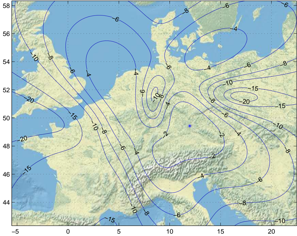
Gain Contours at 450km for FRA. Beam ID=UTC, Polarization=h
