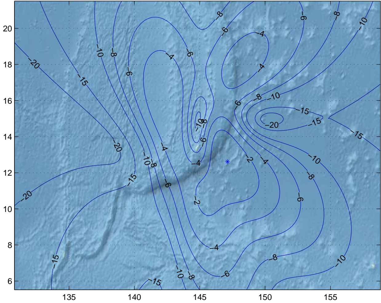
Gain Contours at 450km for GUM. Beam ID=UTC, Polarization=h
