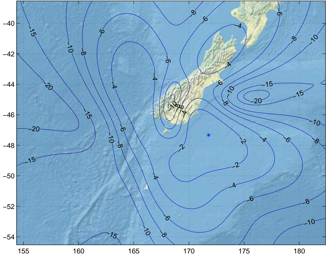
Gain Contours at 450km for IVC. Beam ID=UTC, Polarization=h
