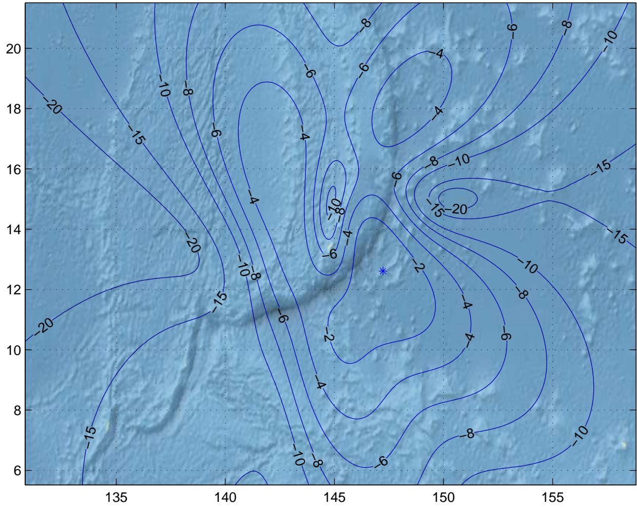
Gain Contours at 460km for GUM. Beam ID=UTC, Polarization=h
