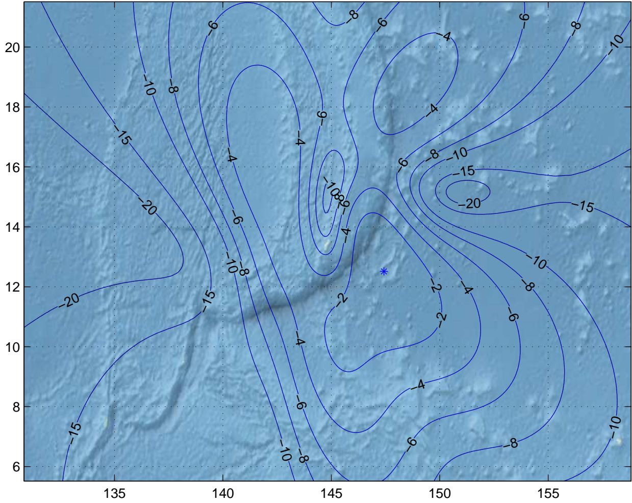
Gain Contours at 505km for GUM. Beam ID=UTC, Polarization=h
