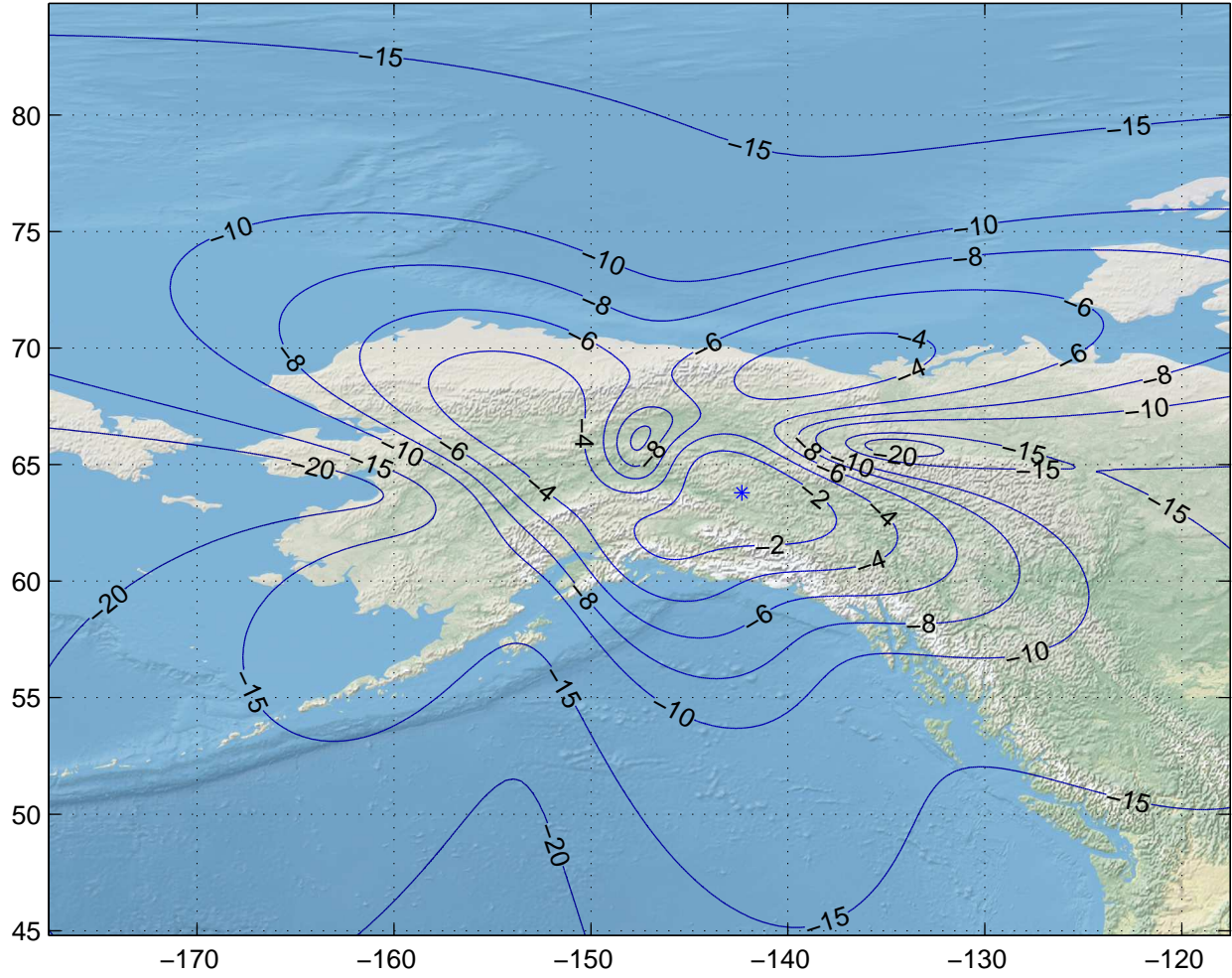
Gain Contours at 450km for FAI. Beam ID=UTX, Polarization=rhcp
