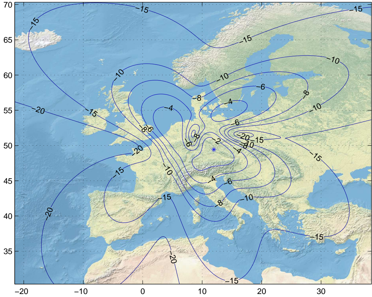
Gain Contours at 450km for FRA. Beam ID=UTX, Polarization=rhcp
