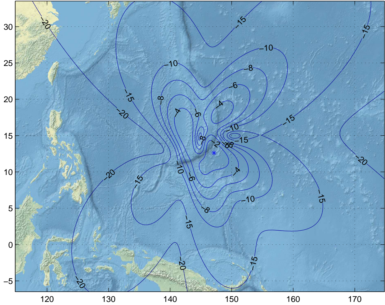
Gain Contours at 450km for GUM. Beam ID=UTX, Polarization=rhcp
