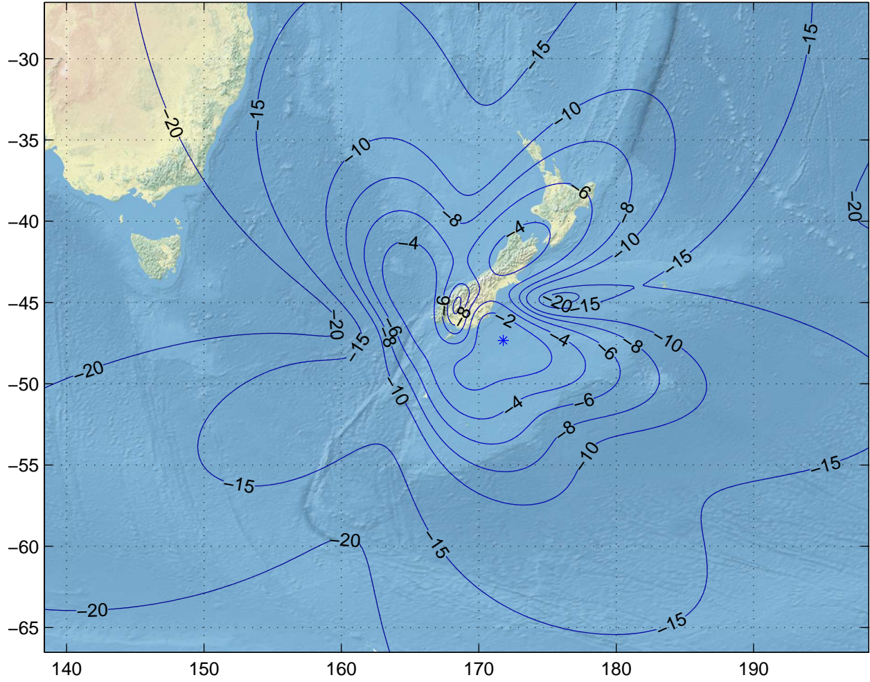
Gain Contours at 450km for IVC. Beam ID=UTX, Polarization=rhcp
