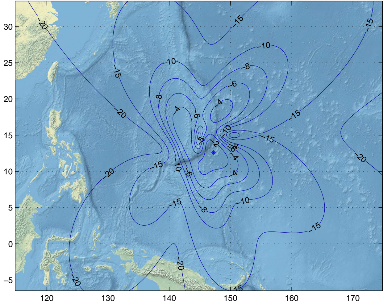
Gain Contours at 460km for GUM. Beam ID=UTX, Polarization=rhcp
